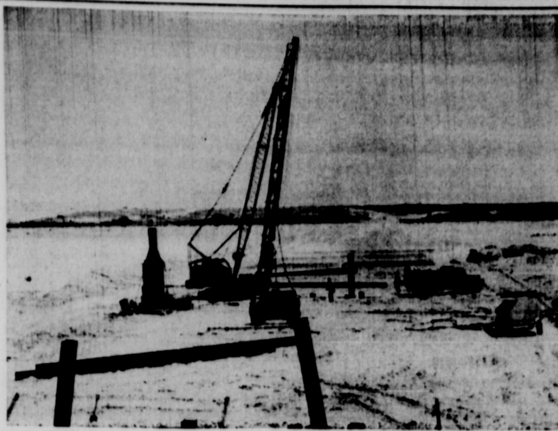
DRIVING PILING—This mammoth machine is driving steel piling for the Canadian River bridge for the state highway 70. The Frost Construction Co. of Hydro, Okla., has the contract for the bridge, due to be finished in 1955.
