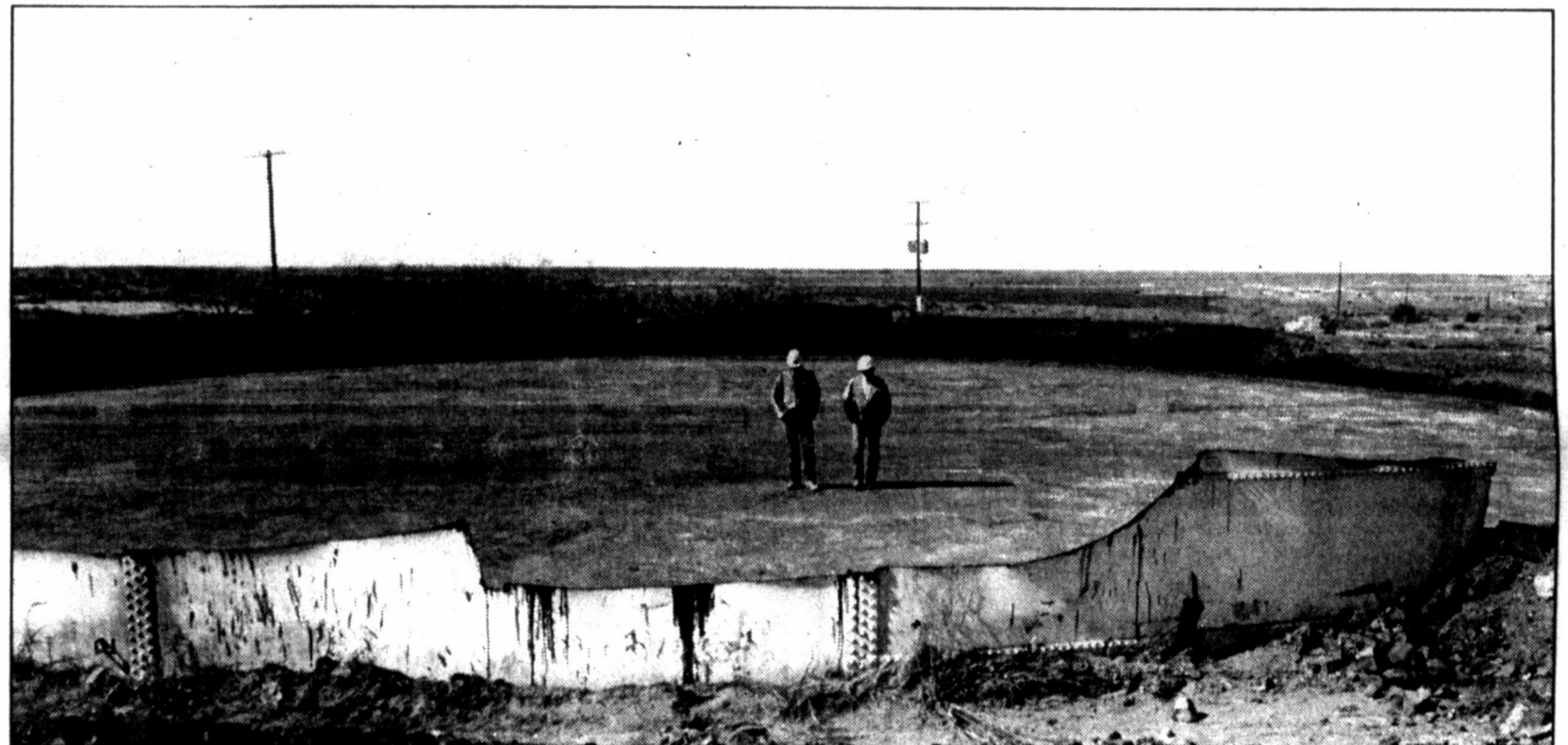
OIL STORAGE was done on a big scale in the 1930's, when this tank was built to store up to 100,000 gallons as a pipeline surge tank. Safety officer Blaine Lemons, left, and consulting engineer Dennis Patton walk its concrete floor. It is being demolished as part of the Col-Tex Refinery cleanup. Its walls were 30 feet high.
