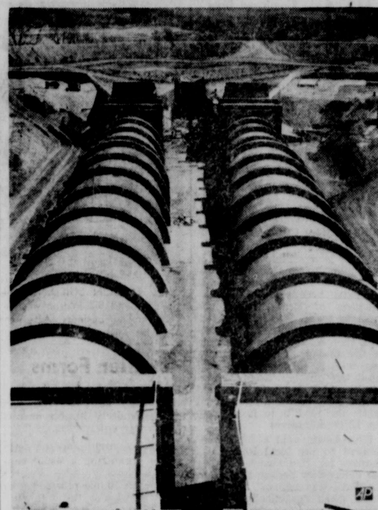
NEW AQUEDUCT—This is a section of a new aqueduct, near San Antonio, a part of the North Concho Reservoir system. Water will flow through these conduits from the North Concho Reservoir to a still basin under construction in the background when North Concho Dam is completed. (P) Photo
