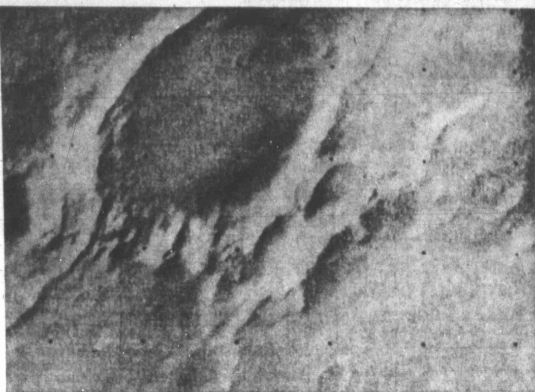
SCIENTISTS CALL IT 'GIANT'S FOOTPRINT'—These two oblique craters near the south polar cap of Mars impelled scientists at Jet Propulsion Laboratory to refer to them jokingly as a giant's footprint and the only evidence they'd see yet of life on the planet.
