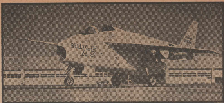
WHAT NEXT? WHY MOVABLE WINGS! —Newest plane to write headlines in the sky is the 10,000 pound Bell X-5, an experimental aircraft with sweptback wings that can be moved during flight. For takeoff, quick climb and landing, the pilot can adjust the wings to a forward position. Test flights at Edwards Air Force Base, Murco, Calif., will demonstrate the pilot's ability to increase his speed at high altitudes by adjusting the wing's sweep-back.
