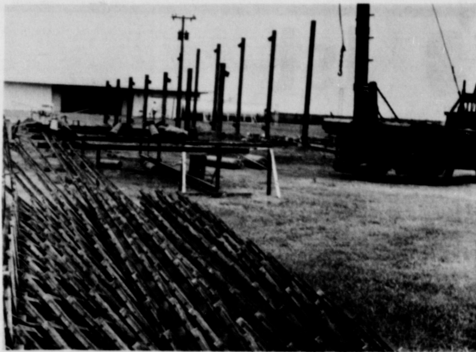
WORK HAS BEGUN on the new Wolverine Stadium at Springlake Schools. The Steel Cross sections are forming the skeleton for the modernistic structure to house Wolverine fans this year. It is scheduled to be completed in time for the first home game of the season with Seagraves on September 11.
