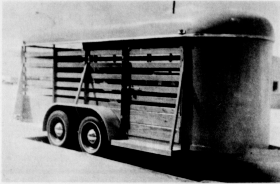
MEMBERS OF THE AG, II CLASSES of the Springlake-Earth School have completed building a sixteen foot stock trailer. The boys have put in eight weeks of work time on this project. The approximate cost of the trailer was $730.00. The trailer was built for Tommy Alair who furnished the materials for the project.
