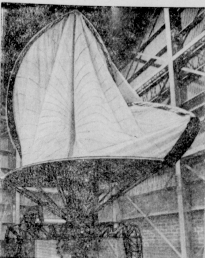
LOLLIPOP RADAR —Resembling a giant lollipop, the Parabolon radar antenna, above, is literally blown up like a balloon. The lightweight, mobile radar unit, designed for the Air Force by Westinghouse, can be assembled or dismantled by a crew of nine in several hours, and weighs only 1,690 pounds, compared to 10,000 pounds for equivalent existing metal antennas and their support structures. The Parabolon antenna stands 30 feet high, and, when inflated, forms a double parabolic reflector, coated on one inside surface with vaporized aluminum to reflect radar waves.
