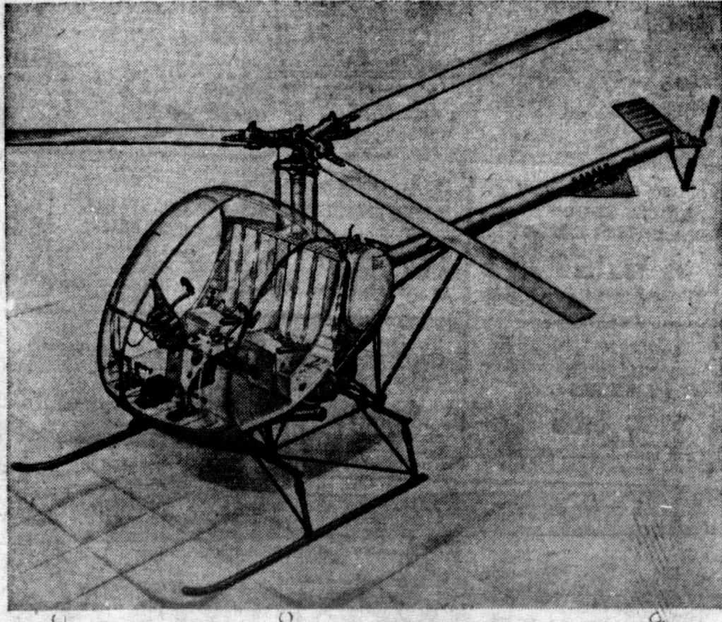
NEW COPTER—Described as "radical in its simplicity and economy," the first five models of this two-man helicopter are being produced for Army evaluation by Hughes Tool Company. It is powered by a 180-hp engine, weighs 890 pounds, and can carry 600 pounds.
