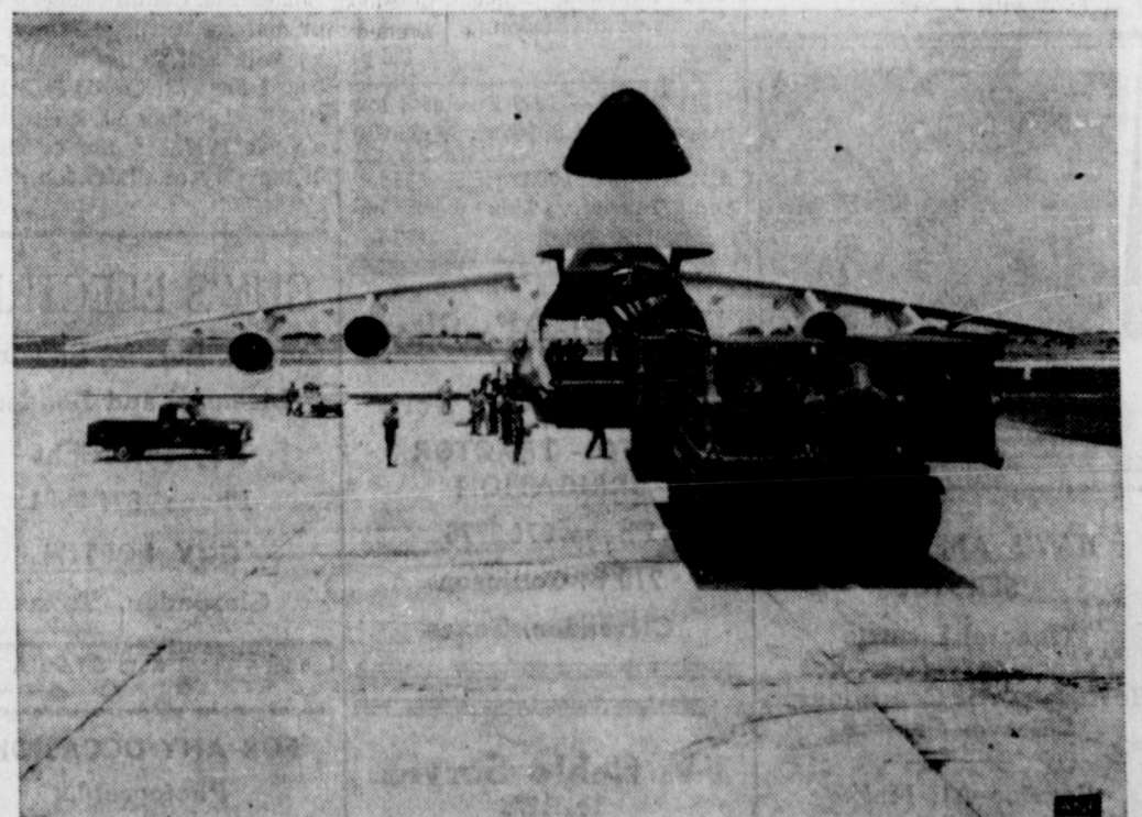
OPEN FOR BUSINESS—Two Army Armored Vehicle Launched Bridges (AVLB) are lined up to enter the cargo compartment of the C-5 GALAXY. No other airplane in the world can load even one—let alone two—of the mobile "scissors" bridge launchers. The two bridges weigh a total of 243,520 pounds. The C-5 offers both front and rear openings, so vehicles can drive straight in one end and out the other, saving ground time. Loading the bridge launchers is part of Army-Air Force rapid response tests at Ft. Hood, Tex.
