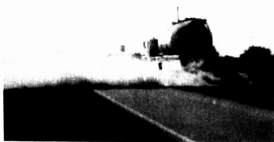
ROAD WORK is continuing on Highway 287 East of Clarendon. The truck at left puts powdered cement on the ground, after which the rototiller-like machine at right incorporates it into the road base. Water trucks then wet down the mixture and big rollers pack the base. Finally, crews spray asphalt to seal the base and top it with hot mix.
