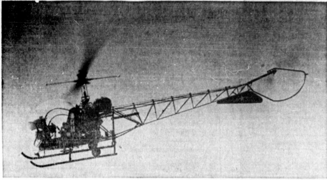
U. S. ARMY'S OH-13 SIOUX helicopter is being demonstrated with a new drone system recently developed by the Bell Helicopter Company, a division of Textron's Bell Aerospace Corporation. The system will give added capabilities to helicopters, especially in the performance of hazardous missions. The drone equipment is installed as a kit and does not disturb the standard manual control system.
