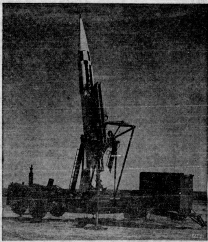
READY AND WAITING—Just minutes after assembly began the SERGEANT ballistic missile sits poised—ready to be fired. Displacement of the launch facilities can be accomplished in an equally short time, fitting the SERGEANT into the Army's "shoot and scoot" concept of tactical warfare. The SERGEANT system's air transportability and quick loading and assembly was demonstrated at White Sands Missile Range, N.M., October 24, when for the first time the SERGEANT was fired by a U. S. Army tactical unit.
