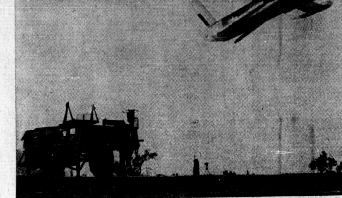
FIRST PHOTO of successful flight test of the combat surveillance drone SD-2 shows rocket-aided high-speed take-off from launching vehicle at the U. S. Army test station, Yuma, Ariz. Controlled from a remote point on the ground, the drone can scout enemy positions, use photography, television or other electronic devices to send or bring back information, then land by parachute without an airport.
