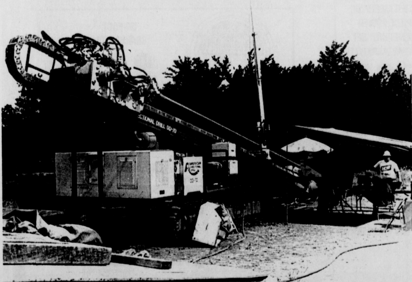
A SOPHISTICATED computer-controlled directional boring machine is used to bore a hole approximately 800 feet long and 15 feet under the Wichita River at FM 368. The project by Lone Star Gas is to replace more than 30 miles of line that was installed in the 1920s from Wichita County to just west of Jean in Young County. The line provides natural gas to a number of communities in Wichita, Archer and Young counties.
