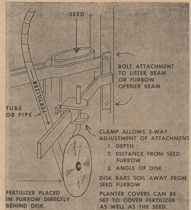
Disk Type Fertilizer Applicator For Row Crop Planters.
