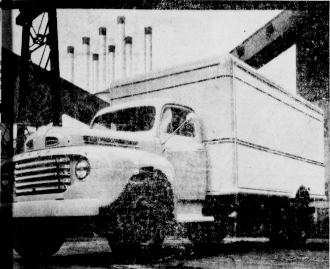
The new 1948 series F-8 Ford 3-ton truck with 195-horsepower is the largest truck ever built by the Ford Motor Company. The new 1948 truck line offers a range of models and capacities than ever before. They are powered by three new truck engines—a 95-horsepower six-cylinder engine, a 100-horsepower V-8 and a 145-horsepower V-8.
