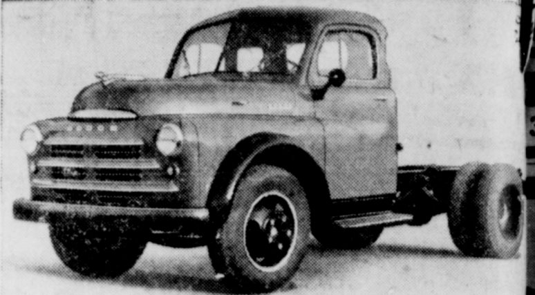
Among the 248 basic gross vehicle weight chassis models just announced in the new Dodge "Job-Rated" truck line is the B-1-H tractor of 128-inch wheelbase, 15,500 pounds gross vehicle weight (1½-ton nominal rating) and 28,000 pounds gross trailer weight. The trucks have many new features.
