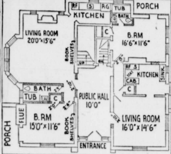
The floor plan (above) illustrates how the first floor was converted into two apartments with a central public hall.
