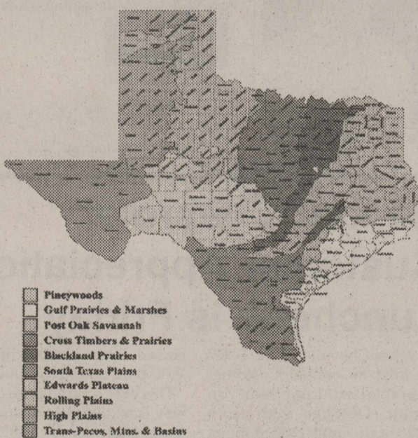
Texas Ecoregions Map
