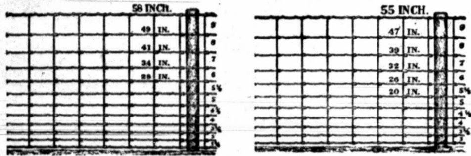
Regular Style Stays 12 in. or 6 in. apart Special Hog, Horse and Cattle Style Stays 12 in. or 6 in. apart
