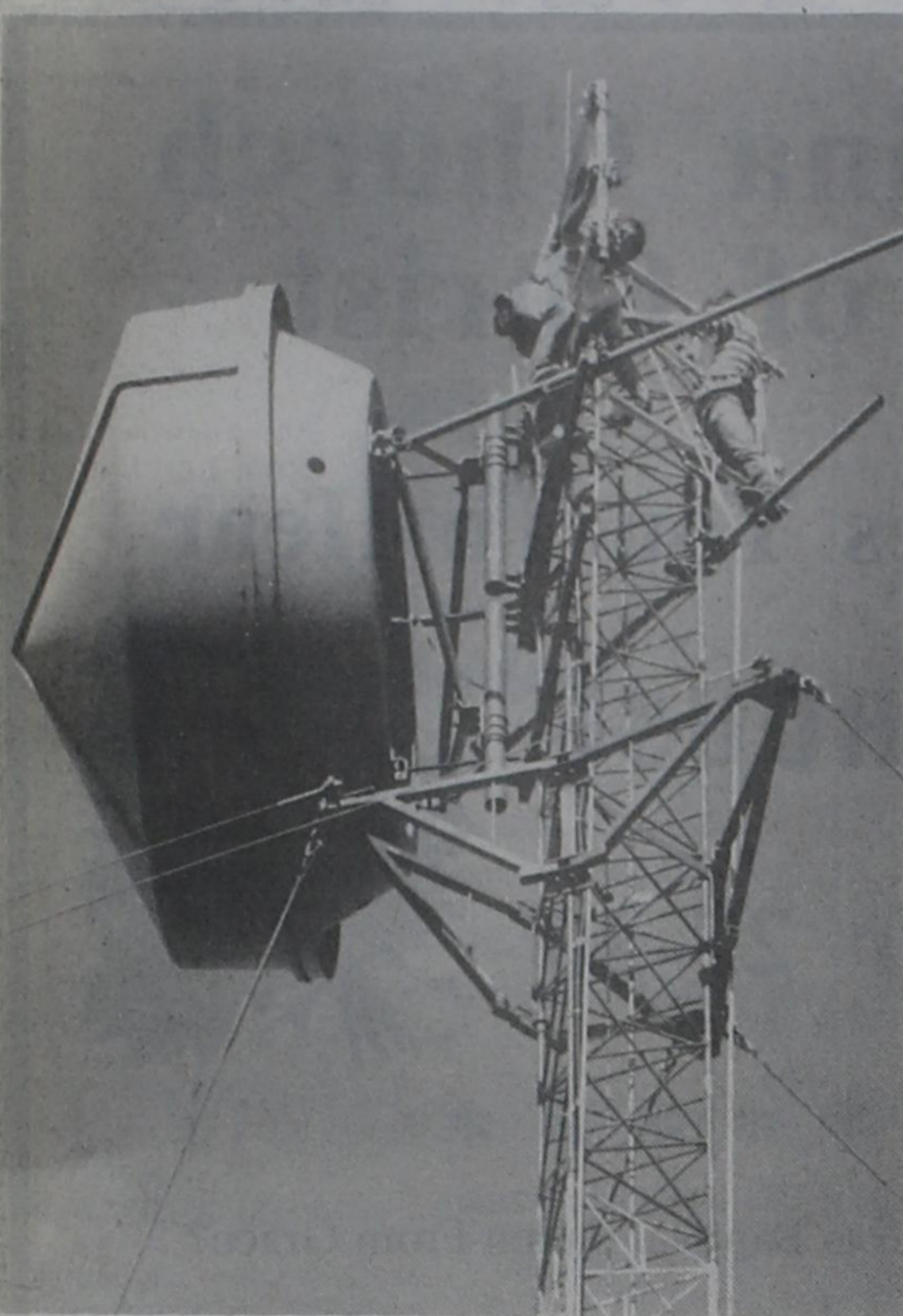
UP SHE GOES....Brad Belcher of Clovis and Paul Adams of Farwell bolt brackets in place to hold cellular telephone antennas high atop an existing tower at the West Texas Rural Telephone central office location at Hub. The antennas provide local cellular telephone service to Parmer County and a large portion of the mid and west Plains. WTRT is a partner in Cellular 3, which is offering cellular telephone service locally.
