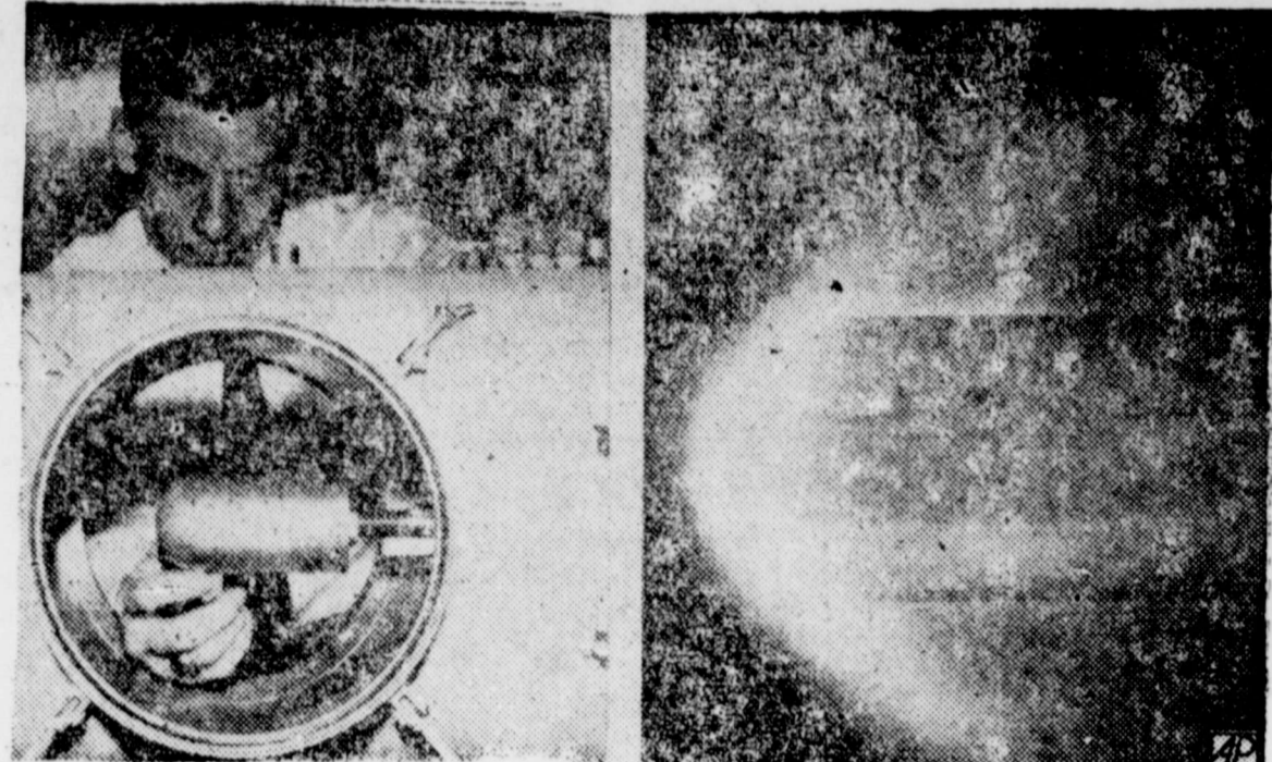
SUPER-SPEED WIND TUNNEL: J. A. Kyser of Chance Vought Aircraft Co., Dallas, left, adjusts a model about to be tested at 10,000 miles per hour in the firm's new "hypersonic" wind tunnel. At right, speed of sound glows brightly as it bends around the blunt nose of the model. (AP Wirephoto).
