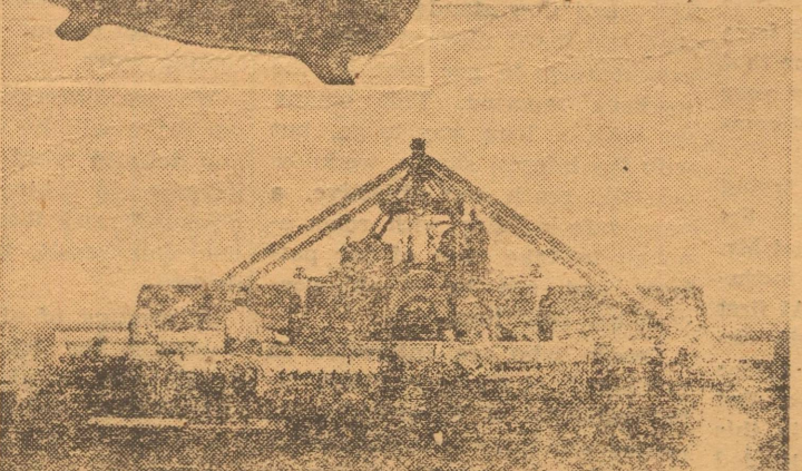
GIANT WHEEL TRACTOR, constructed about 1908 by a predecessor company of Caterpillar, Tractor Co., Peoria, Ill., was one of the largest tractors ever built, measuring over 45 feet wide. Designed to work in soft, peat soils, its wide wheels proved cumbersome and led to the construction of the first practical tractor type in 1904.
