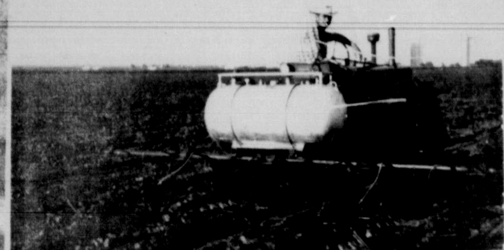
FLAME CULTIVATION--A new way to cultivate in this area, with flame instead of plows, is being demonstrated by Jerry Strawn on a farm near Bovina. Object of the Gotcher flame cultivator is to create, temporarily, a temperature high enough to dehydrate or rupture plant cells which will result in the death of obnoxious vegetation without injury to older and harder cultivated crops. Strawn is operating the new cultivator commercially. They are sold by Charles Oil Co. in Bovina.
