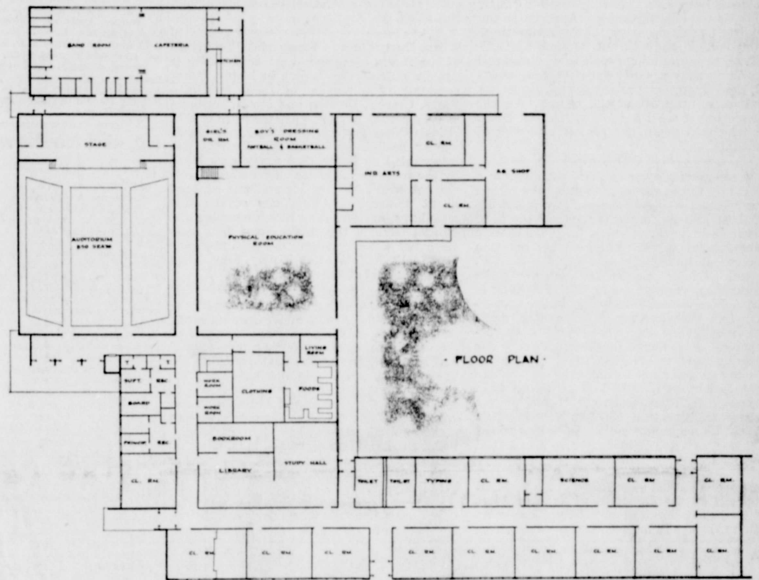
Floor Plan of New Floydada High School Building
