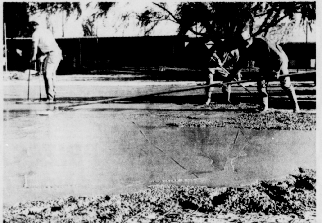
COURT CONSTRUCTION....Lewellen Construction Company began work this week on the new tennis courts at Friona Country Club. Delton Lewellen, right, is shown with other workmen as they smooth out the concrete during the first phase of construction.
