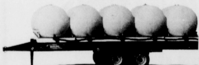
3 The Rhoman "Pup" rigged with a NURSE UNIT.
