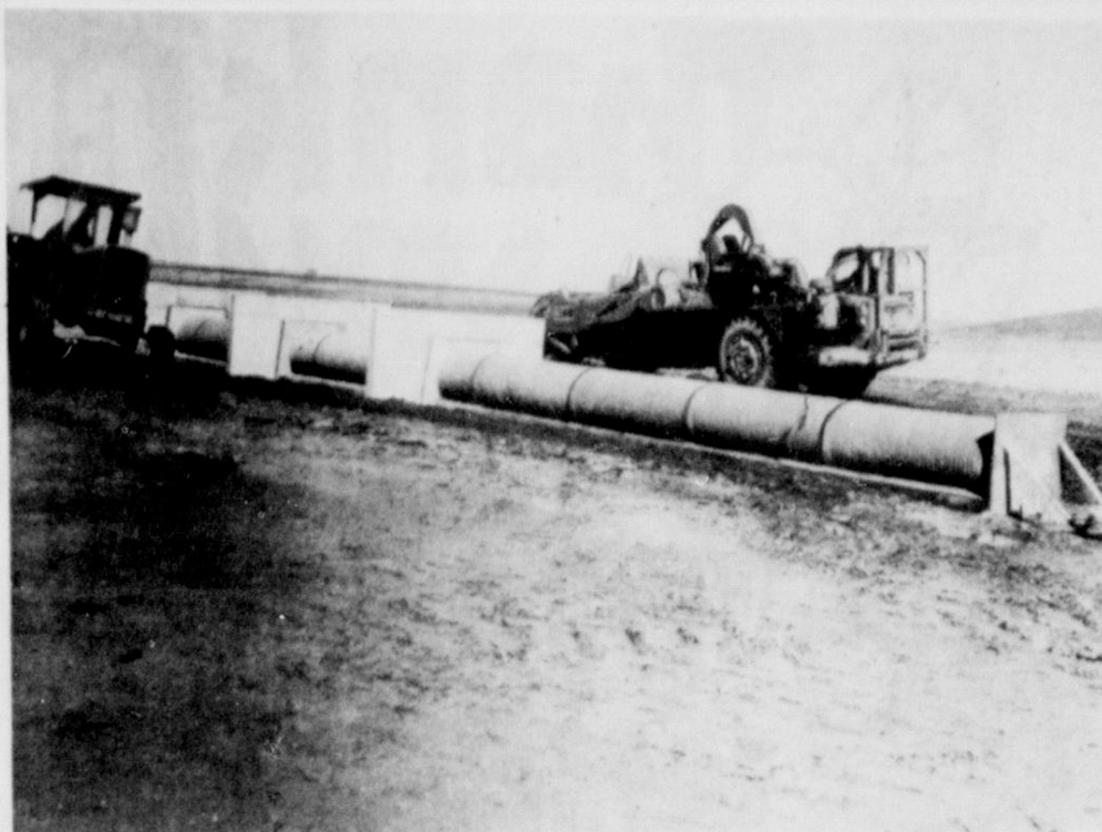
SPILLWAY GOES IN... The three-foot pipe which makes up the spillway at the Catfish Draw damsite north of Bovina is shown
