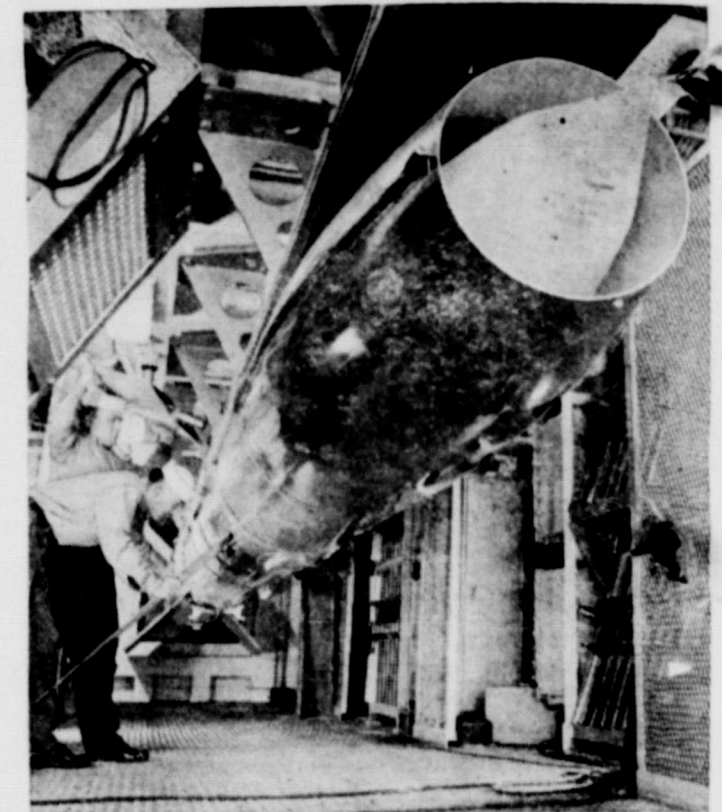
SLEEK NEW SEA MISSILE —A deadly Talos guided missile is checked in aboard the USS Galveston, a missile-cruiser which was commissioned May 28 at the Philadelphia Naval Shipyard. It is the first of a projected fleet of atomic-age fighting ships. The supersonic Talos, made by Bendix Aviation, can destroy enemy aircraft at stratospheric altitudes and has a range of more than 65 miles.
