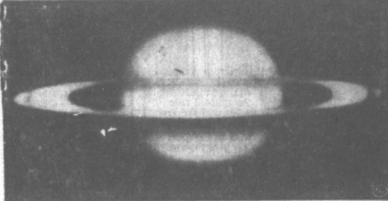
Saturn's ring system appears clearly in this photograph. The rings, which are 171,000 miles in diameter, are only 10 miles in depth. Arranged in three layers, they are composed of minute dust-sized particles, each of which revolves in its own orbit about the mother planet.
