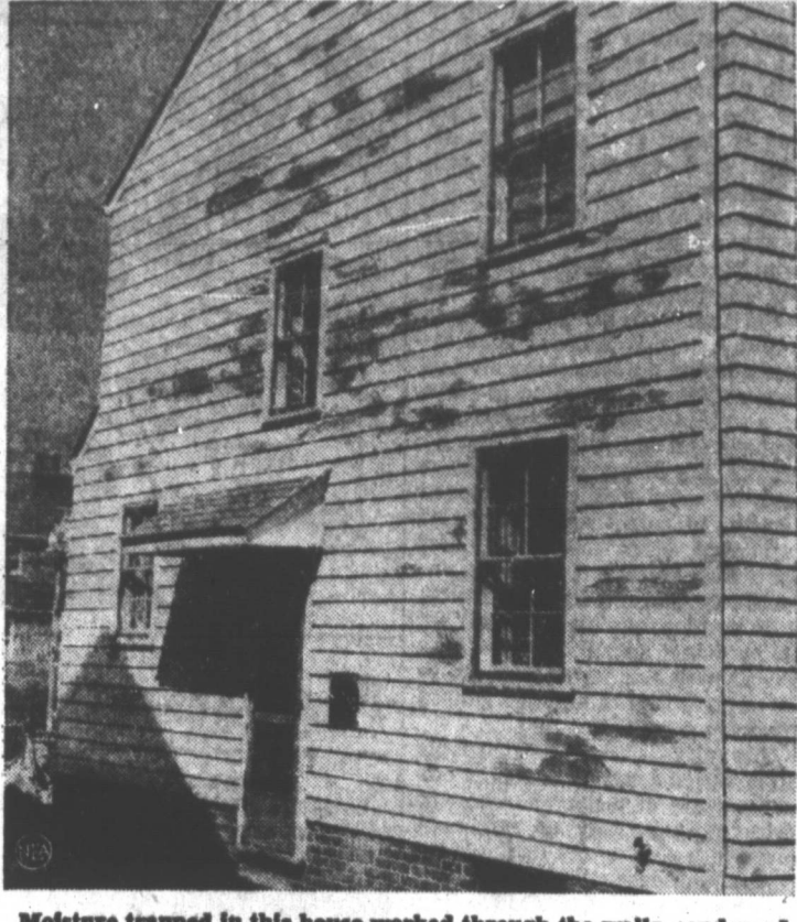
Moisture trapped in this house worked through the walls, condensed into water and caused this scabby peeling of the exterior paint.
