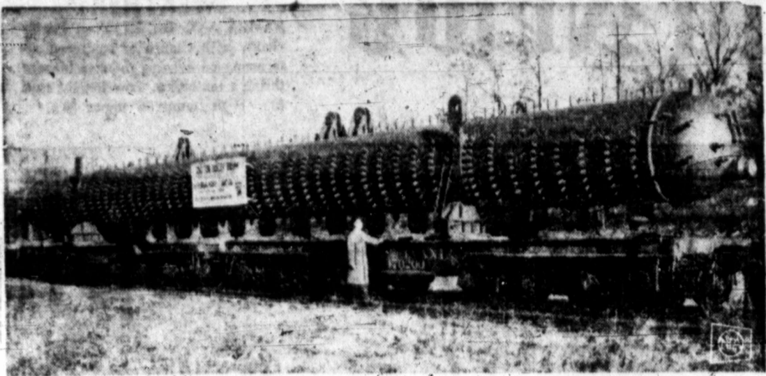
PRICKLY PROBLEM —Securely moored atop two specially designed heavy-duty flat cars, an odd-looking 100-foot drum is given a last-minute check before leaving the Foster Wheeler Corp. plant at Mountaintop, Pa. The prickly boiler is part of a steam generating and condensing installation. Details on how the mammoth load was to be shipped were worked out between manufacturer and rail carrier even before it was built.
