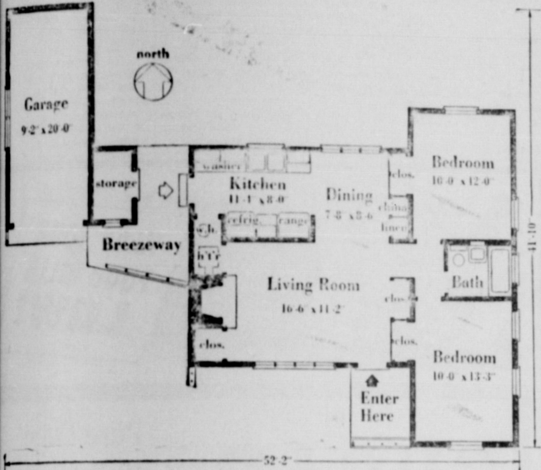
SOUND SIMPLICITY at rock bottom cost is the keynote of this new model home recently opened by the Montauk Beach Company, Inc., on Long Island, N. Y. Designed after the suggestions of Douglas Younger, building consultant for Good Housekeeping magazine, the architect kept expenses down by: (1) Elimination of basement; (2) Simple frame and roof; (3) Dry Wall construction; (4) Simplified doors and trim; (5) Use of closets for partitions. Although the house embodies the latest principles and advancements in moderate priced design and construction, it's so simple to build that the tool-wise amateur can do much of the work. The Montauk House lends itself to any seashore terrain and can be used for a summer or year round home. It is featured in the June issue of the magazine.
