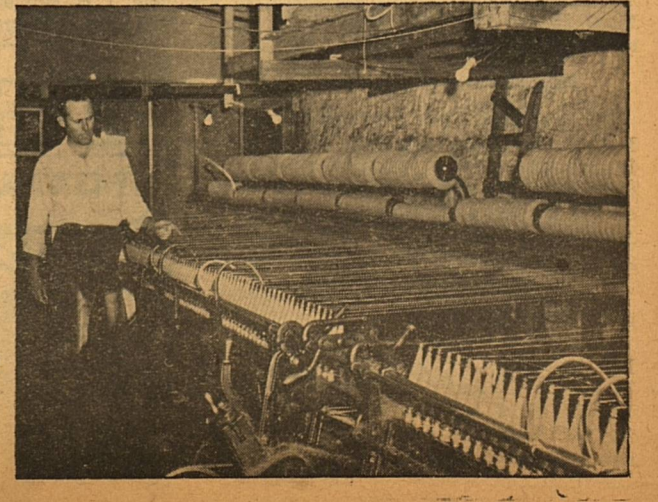
Texas' only wool blanket mill is at Eldorado. Owner Joe Christian points to the complicated spinning machine.
