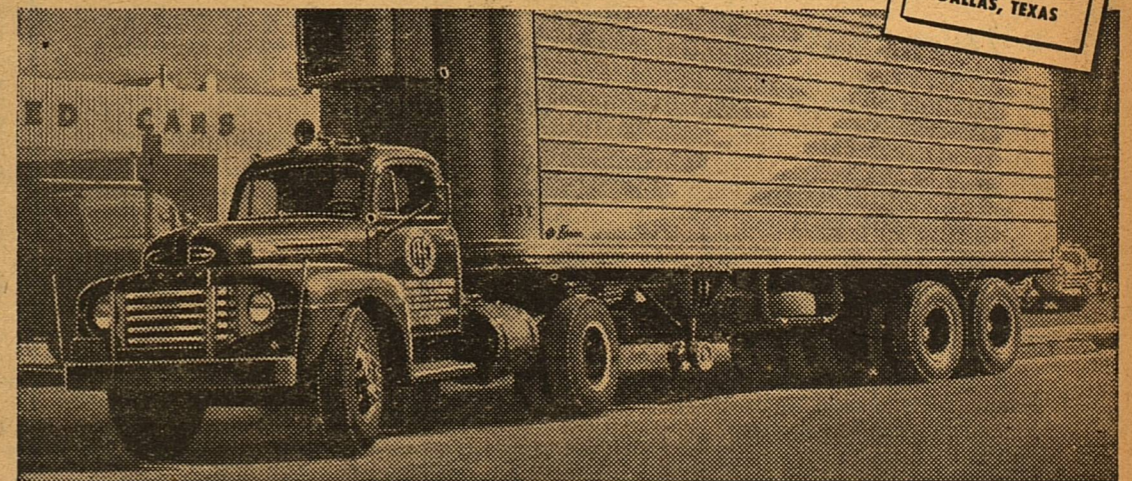
Ford Model F-7 BIG JOB shown has a Gross Combination Weight rating of 35,000 lbs. as a tractor; Gross Vehicle Weight rating of 19,000 lbs.
