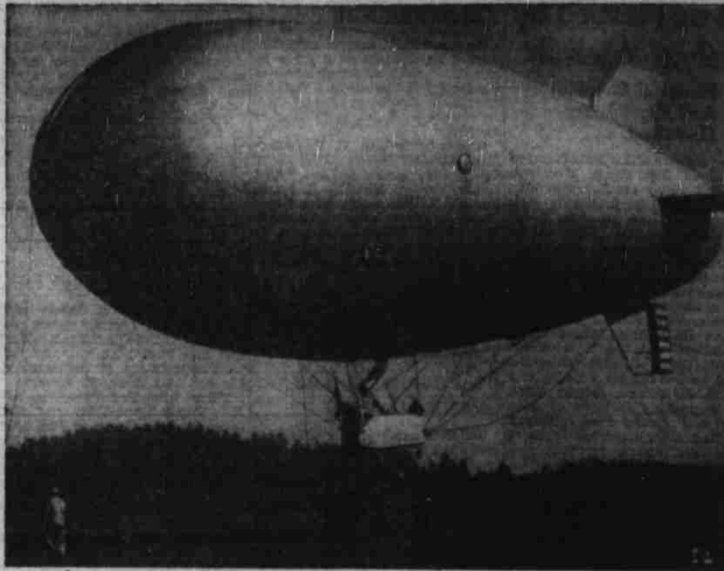
ARMY'S NEW COMBINATION BLIMP and captive balloon, given a test at Fort Lewis, Washington, carries a crew of two persons, and is handled by a ground crew of nine. Inflated with helium gas, the non-rigid blimp is equipped with a small control car containing a 30-horsepower motor. The control car can be replaced by a basket and cable, and the balloon used as a captive for artillery fire observation. This picture was made as the blimp was taking off.
