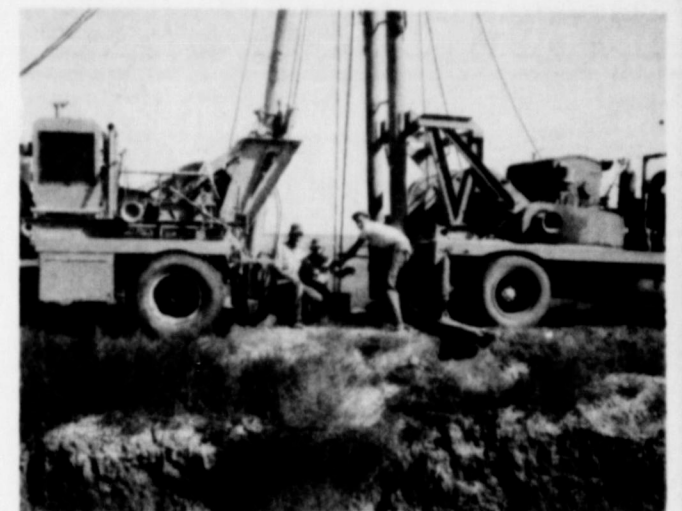
PERFORATING CASING IN THE NEW DEVELOPED HOLE
