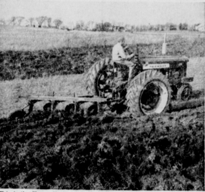
This is the Farmall 450 in the new 1957 farm tractor line now being shown by International Harvester dealers everywhere. The "450" is shown here with the new Fast-Hitch with Traction Control pulling the new McCormick four-bottom plow.
