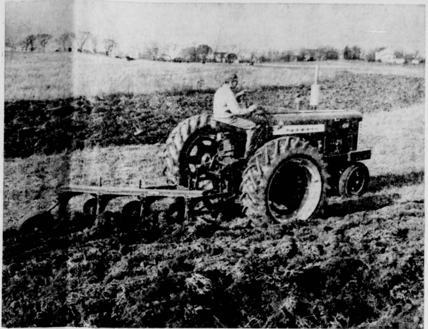
This is the Farmall 450 in the new 1957 farm tractor line now being shown by International Harvester dealers everywhere. The "450" is shown here with the new Fast-Hitch with Traction Control pulling the new McCormick four-bottom plow.
