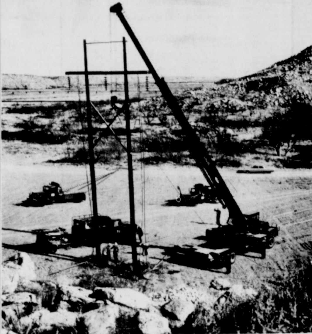
SECOND IN NATION - An 80 foot electric transmission line structure can be lifted and set into place in 8-1/2 minutes with Southwestern Public Service Company's new hydraulic crane. The unit, the second one to go into service in the nation, was specifically designed for use in the
