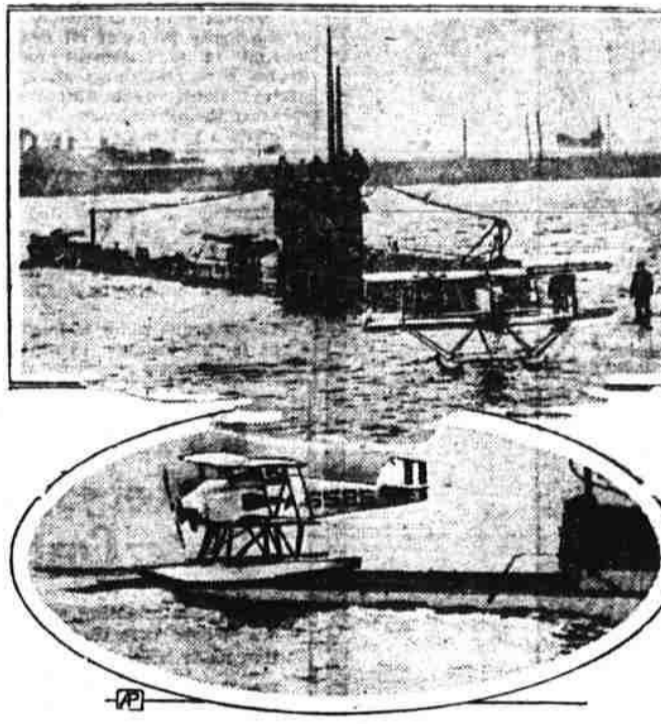
The navy's new folding wing seaplane will be an advanced step over a tiny scout (below), shown assembled for flight from a submarine's deck tank. Top shows undersea boat partially submerged to receive scout plane.
