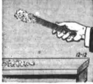
A hard rubber comb, after being rubbed, will attract bits of paper.
