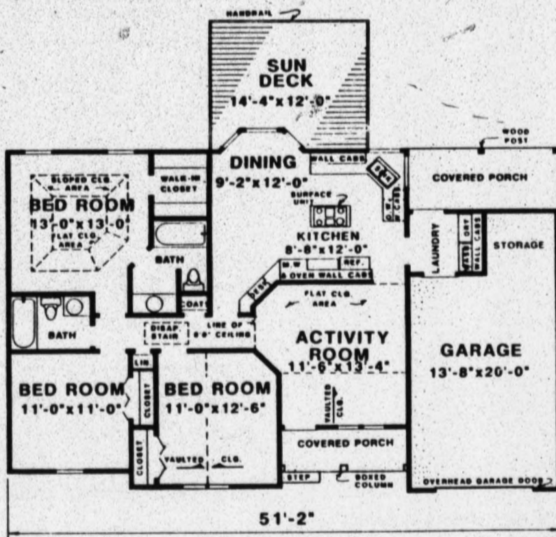
FLOOR PLAN
