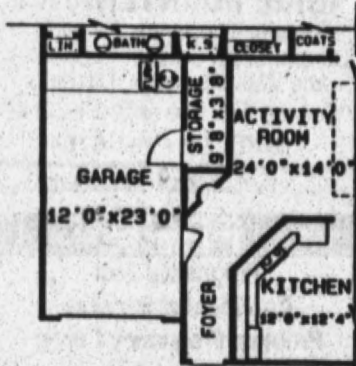
ALT. FLOOR PLAN FOR SLAB FOUNDATION
