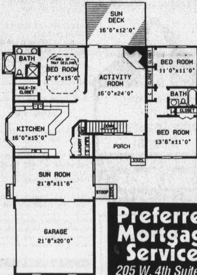
FLOOR PLAN
