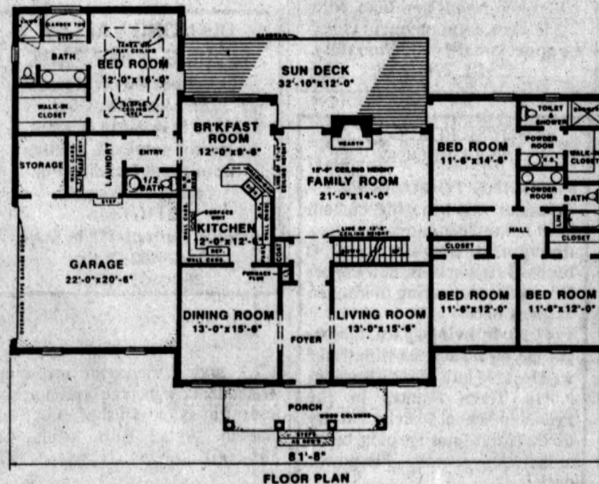
FLOOR PLAN
