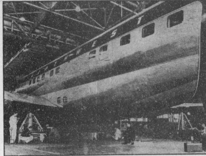
Too large to be weighed on a single scale, this Boeing Stratocruiser is balanced on three—one under the nose, and two at the wing-roots. The plane's wheels are a scant inch off the floor of this building at Boeing's Seattle, Wash., headquarters. By adding the figures registered on each of the three scales, the total weight of the plane—71 tons—is computed.
