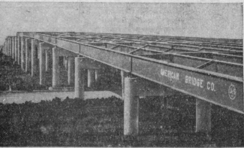
This rising steel and concrete structure over Calhoun Road in Houston, Texas, will carry the heavy traffic of the new Galveston-Houston express highway through the Texas metropolis' booming East End. A 1,192-foot structure, this overpass comprises one of five in Houston's East End, the steel for which is being furnished by the American Bridge Company, subsidiary of United States Steel. The 50-mile expressway, termed among highway builders as "the highway of tomorrow," will be the ultimate in new highway construction in Texas, a state already famed for its fine highway system.
