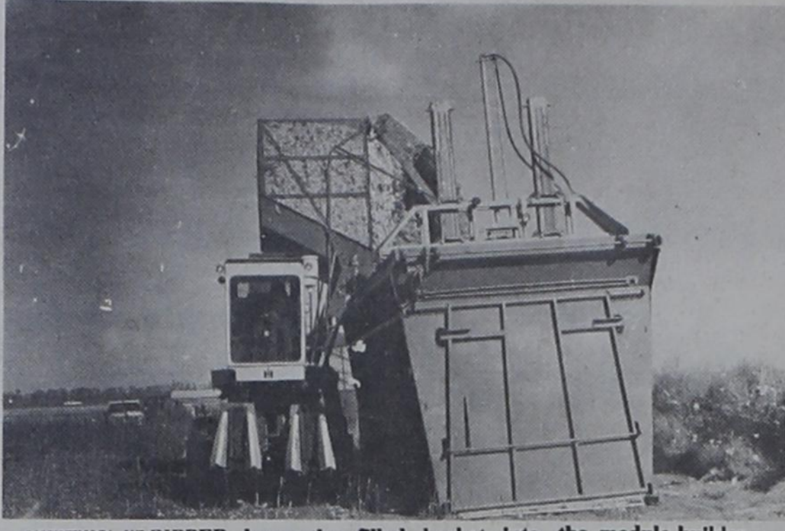
COTTON STRIPPER dumps the filled basket into the module builder. An operator in a cab manipulates the controls which cause the cotton to be pressed tightly.
