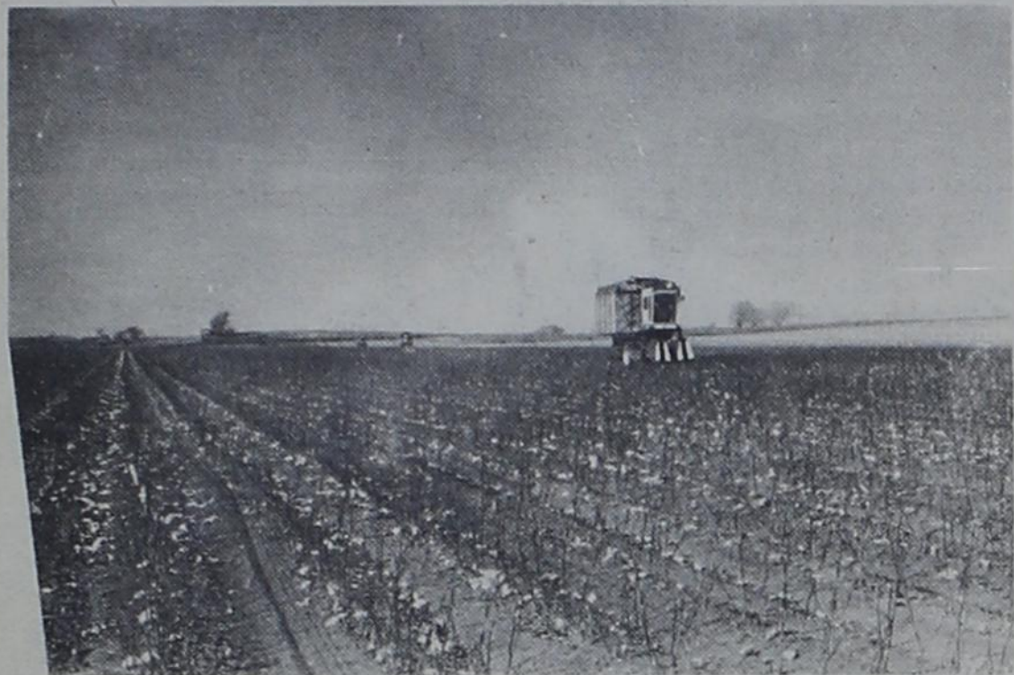
THE LEAD cotton stripper with filled basket moves across the field toward the module builder. Pictured in the background are three other strippers gathering cotton.
