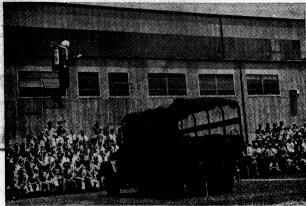
DEMONSTRATING THE "FLYING BELT." Using the experimental Small Rocket Lift Device (SRLD), believed to be the first portable rocket equipment to carry man in individual controlled free flight, a test engineer soars over a truck during the recent Project Mobility demonstrations at Ft. Eustis, Va. In previous tests, the experimental "flying belt," developed by Bell Aerosystems Co., Buffalo, N. Y. for the U. S. Army Transportation Research Command, has flown at a speed of 20 mph and has made lateral flights of up to 360 feet.
