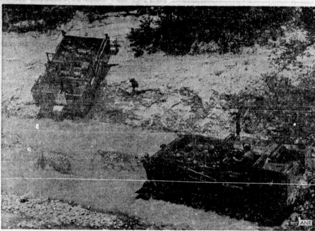
VERSATILE COMBAT TRACTOR FOR ENGINEERS — Two experimental "Universal Engineer Tractors" undergo tests at Fort Belvoir, Va. As well as serving as bulldozer, grader, scraper, dump truck, prime mover and cargo carrier, the machine can carry a squad of combat engineers over rough terrain at speeds up to 30 MPH. The U. S. Army Mobility Command's Engineer Research and Development Laboratories have awarded the International Harvester Company a contract to produce six more experimental models for testing in the field.
